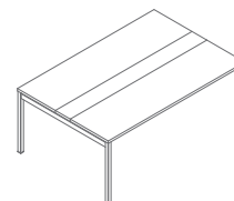
SY48 1800 / 1210 / 740 64.7 kg
