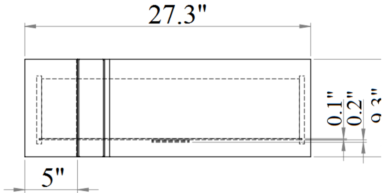
Front View
