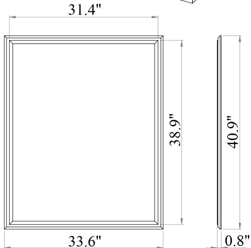
Front View
