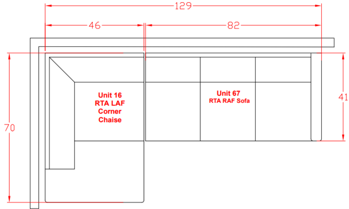
617 Configuration 2 Space Between Units = 3/4" For Connecting Brackets Unit is 3" Away From Wall
